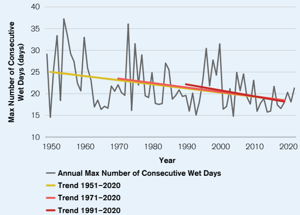
FIGURE 7B. Mozambique's Historical Annual Maximum Number of Consecutive Wet Days, Along with Decadal Trends for Various Periods between 1951 and 2020, based on ERA5 Data
