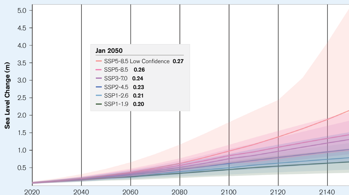
FIGURE 8. Projected Total Sea Level Change Under Different SSP Scenarios Relative to the Historical Baseline (1995–2014). The Shaded Ranges Show Uncertainties at 17th–83rd Percentile Ranges. Data from NASA 14 .
