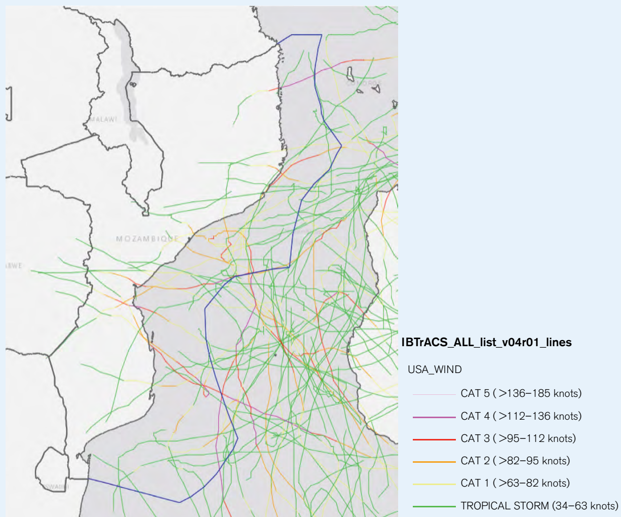
FIGURE 9. Observed Historical Cyclones from IBTrACS 21 . All Recorded Cyclones have been Classified According to the Saffir-Simpson Scale Using the Variable “USA_wind”, which Records Sustained Maximum Winds Every 3 Hours (see label in knots). The IBTrACS Historical Data Covers Cyclones Recorded from 1840 to 2023, with the Caveat that Records Prior to 1980 may be Incomplete.
