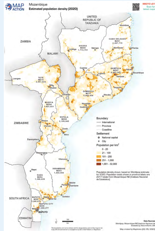
FIGURE 1B. Estimated Population Density (population per square km), 2020 5
