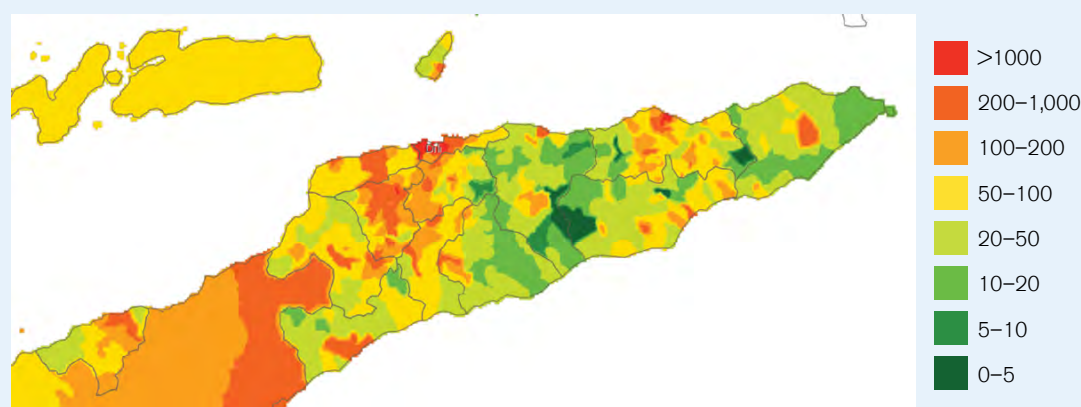
FIGURE 2B. Population Density (per square km), 2020 5
