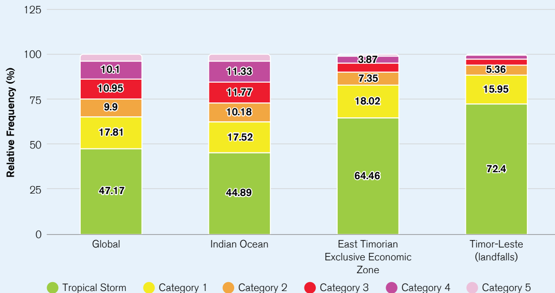
FIGURE 13. Simulated Percentage of Cyclone Types for Global Oceans, Indian Ocean, East Timorian Exclusive Economic Zone, Timor-Leste (landfalls), CHAZ, Historical Simulation (1951–2014)
