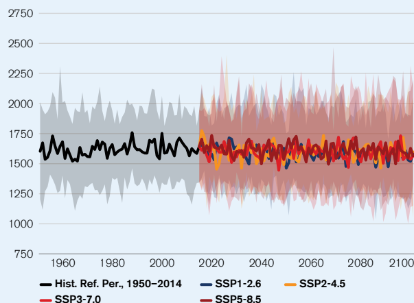
FIGURE 8. Projected Annual Precipitation for Different Climate Change Scenarios as Labeled, Along with the 10th–90th Percentile Dispersion Across Models
