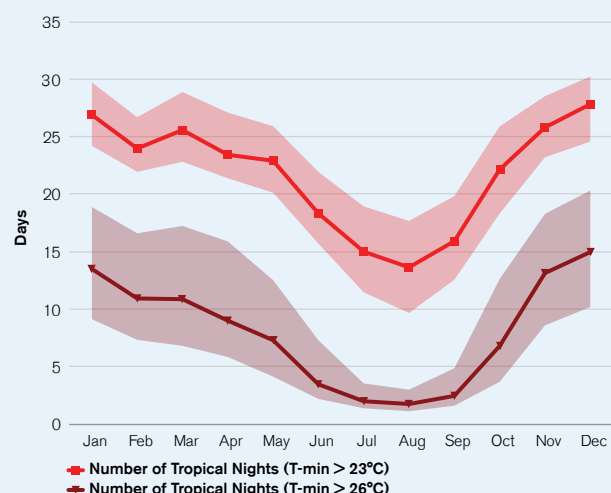
FIGURE 9B. Projected Monthly Number of Tropical Nights at Different Temperature Thresholds by 2080–2099 Under SSP3-7.0
