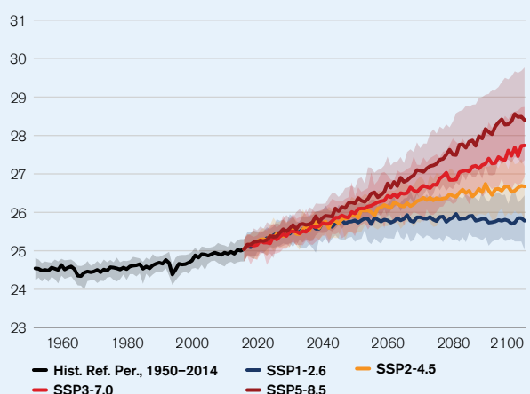
FIGURE 6. Projected Average Mean Surface Air Temperature for Different Climate Change Scenarios as Labeled, Along with the 10th–90th Percentile Dispersion Across Models
