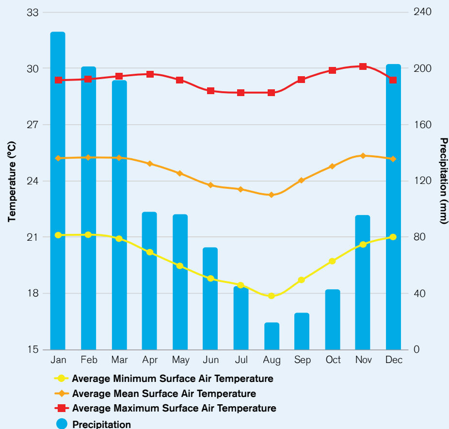
FIGURE 3. Monthly Historical Climatology of Average Temperature (minimum, average, and maximum) and Total Precipitation (1991–2022) for Timor-Leste (CRU dataset)
