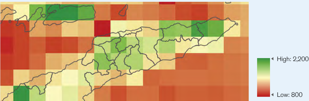
FIGURE 4B. Averaged Annual Total Precipitation (1991–2022) in mm for Timor-Leste (ERA5-dataset). ADM-1 Municipalities are Overlaid.
