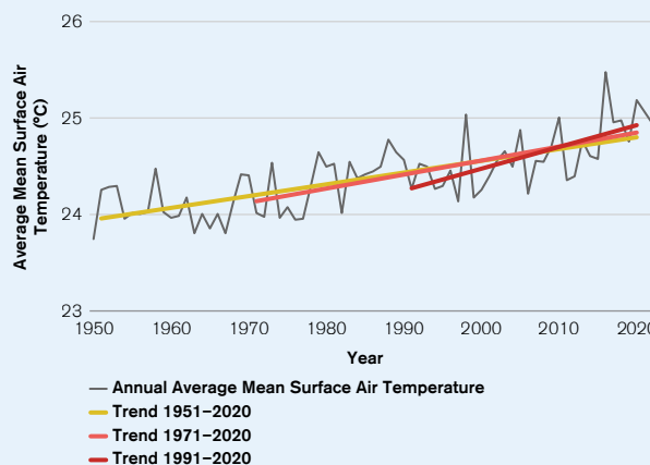
FIGURE 5. Timor's Leste Annual Mean Surface Air Temperature Time Series and Decadal Trends for Different Periods between 1951 and 2020 as indicated, ERA5 Data
