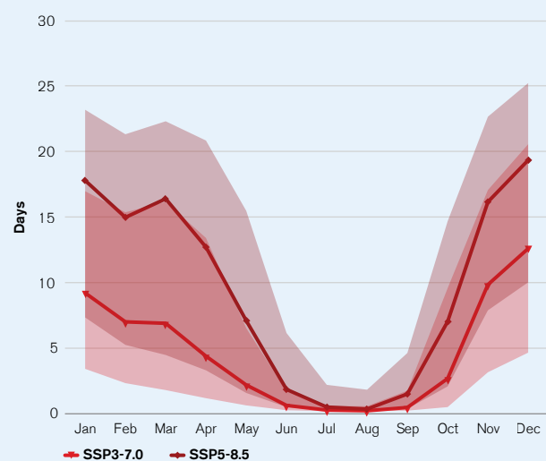
FIGURE 10. Projected Monthly Climatology of Number of Days with Heat Index > 35^{\circ}\text{C} by 2080–2099 Under SSP3-7.0 and SSP5-8.5
