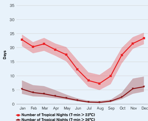
FIGURE 9A. Projected Monthly Number of Tropical Nights at Different Temperature Thresholds by 2040–2059 Under SSP3-7.0
