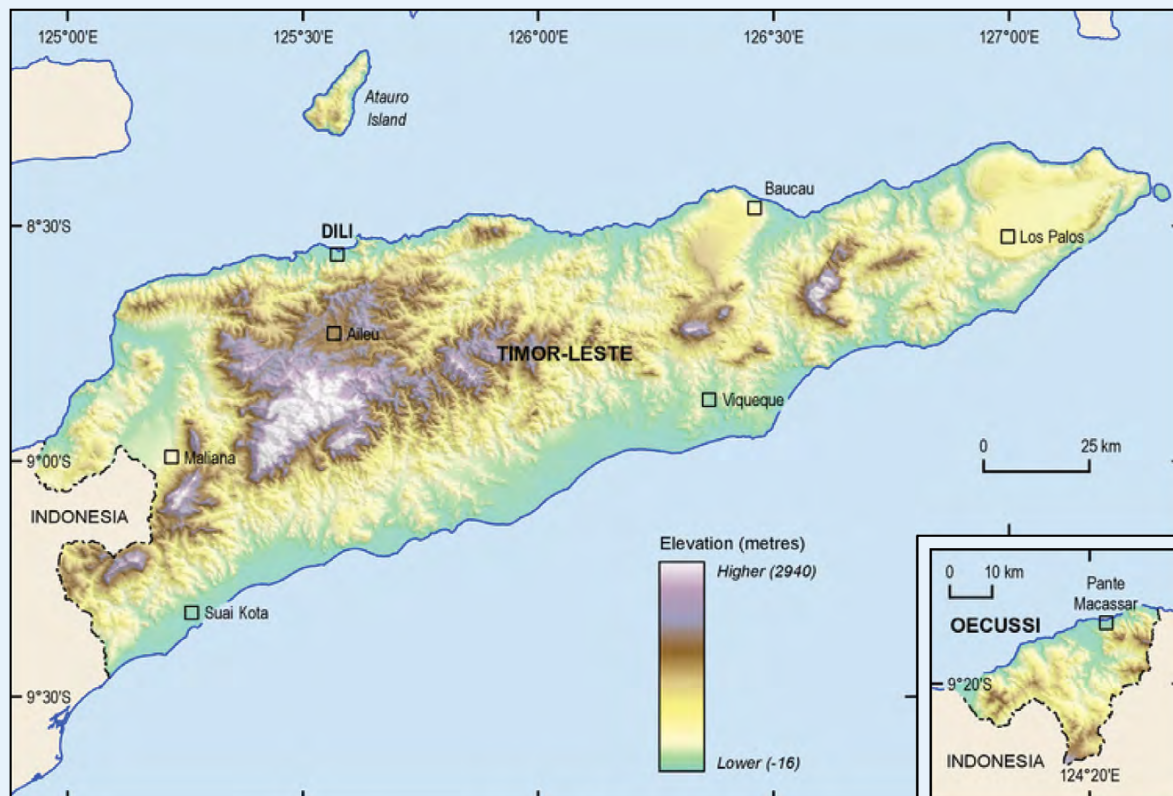
FIGURE 1. Topography of Timor-Leste (in meters) 4 . The Island's Topography Plays a Crucial Role in Shaping Wind Patterns, Climate, and the Impacts of Sea Level Rise. The Municipality Oecussi is Located within West Timor.
