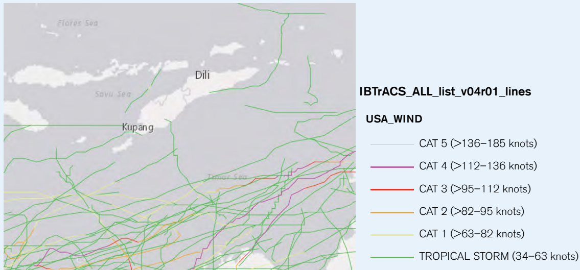
FIGURE 12. Observed Historical Cyclones from IBTrACS 31 . All Recorded Cyclones have been Classified According to the Saffir-Simpson Scale using the Variable “USA_wind”, which Records Sustained Maximum Winds Every 3 Hours (see label in knots). The IBTrACS Historical Data Covers Cyclones Recorded from 1840 to 2023, with the Caveat that Records Prior to 1980 may be Incomplete. Note that Most Cyclones Occur South of East-Timor.
