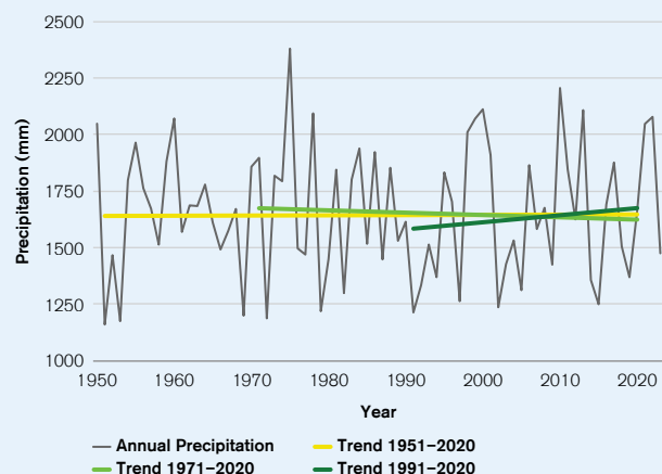
FIGURE 7. Timor-Leste's Annual Precipitation Time Series and Decadal Trends for Different Periods between 1951 and 2020 as Indicated, ERA5 Data
