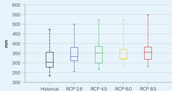
FIGURE 8. Projected average annual precipitation for the Kyrgyz Republic in the period 2080–2099. 17
