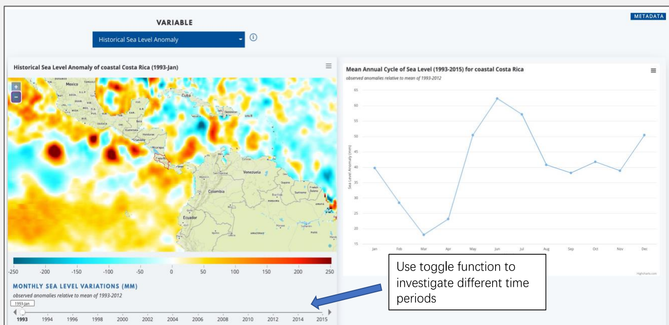
Figure N. Observed Sea Level Anomaly for Coastal Costa Rica; observed anomalies relative to mean of 1993-2012
