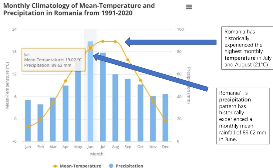
Figure E. Seasonal Cycle of Monthly Mean Temperature and Precipitation in Romania (1991-2020)
