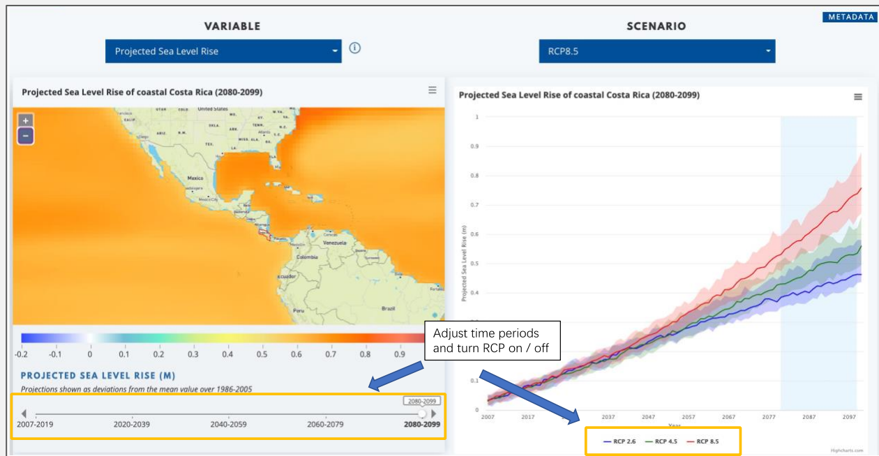
Figure O. Projected Sea Level Rise, Coastal Costa Rica; projection values as deviations from mean value 1986-2005
