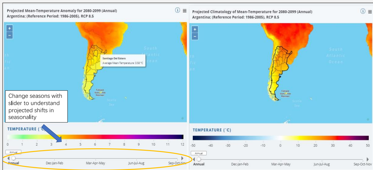
Figure G. Spatial Variation and Change; anomaly (left) and mean (right)
