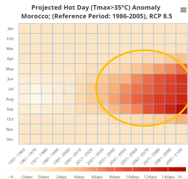
Figure K. Projected Change in Number of Hot Days in Morocco
