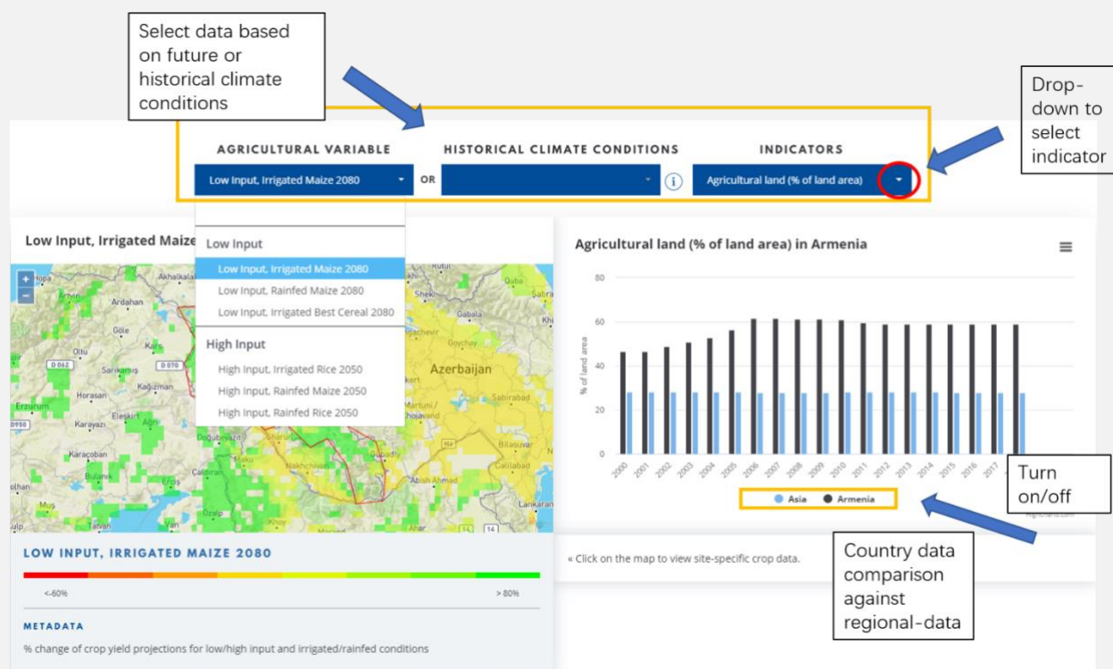
Figure M. Climate Change Impacts on Agriculture Indicators Uruguay (Agricultural Variable)
