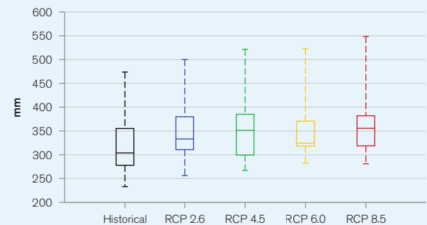
FIGURE 8. Projected average annual precipitation (mm) for Kazakhstan in the period 2080–2099. 21
