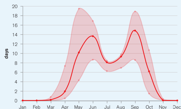
FIGURE 6. Projected change in Summer Days (Tmax >25°C) 23
