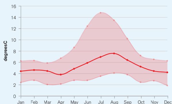
FIGURE 9. Projected average daily max temperature for Croatia 52
