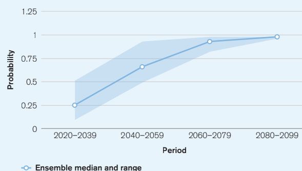
FIGURE 5. Projected change in probability of heat waves in FSM under RCP8.5 (compared to 1986–2005) 2
