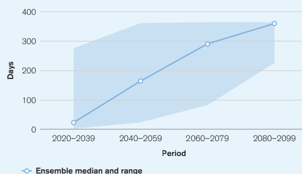
FIGURE 6. Projected change in the count of days in which climate conditions breach the Heat Index >35°C threshold, under RCP8.5 2
