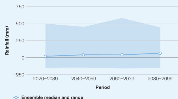
FIGURE 9. Projected change in annual maximum 5-day rainfall (25-year return level) for FSM, under RCP8.5 2
