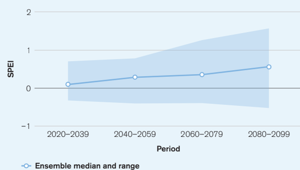
FIGURE 7. Projected change in Annual Mean Drought Index for FSM, under RCP8.5 2
