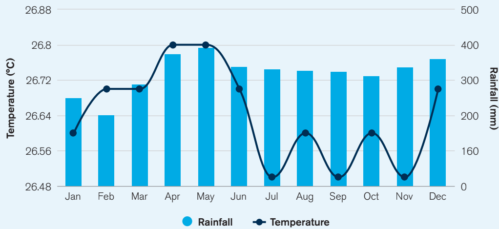
FIGURE 1. Average monthly temperature and rainfall in FSM, 1991–2020 4
