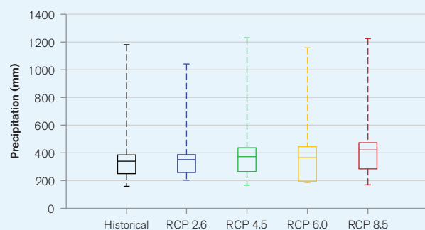
FIGURE 8. 5-day precipitation — historical and projected scenarios of 25-year return level in FSM for period 2040–2059 2
