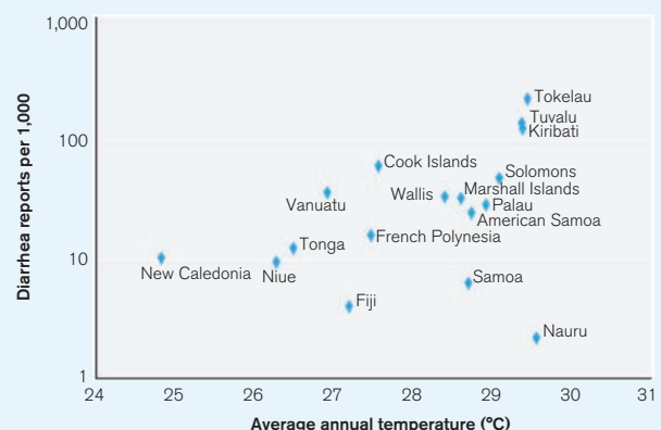
FIGURE 13. Annual average temperature and average reporting rates for diarrheal disease, Pacific islands (1986–1994). r^2 = 0.49 ; p < 0.05 43
