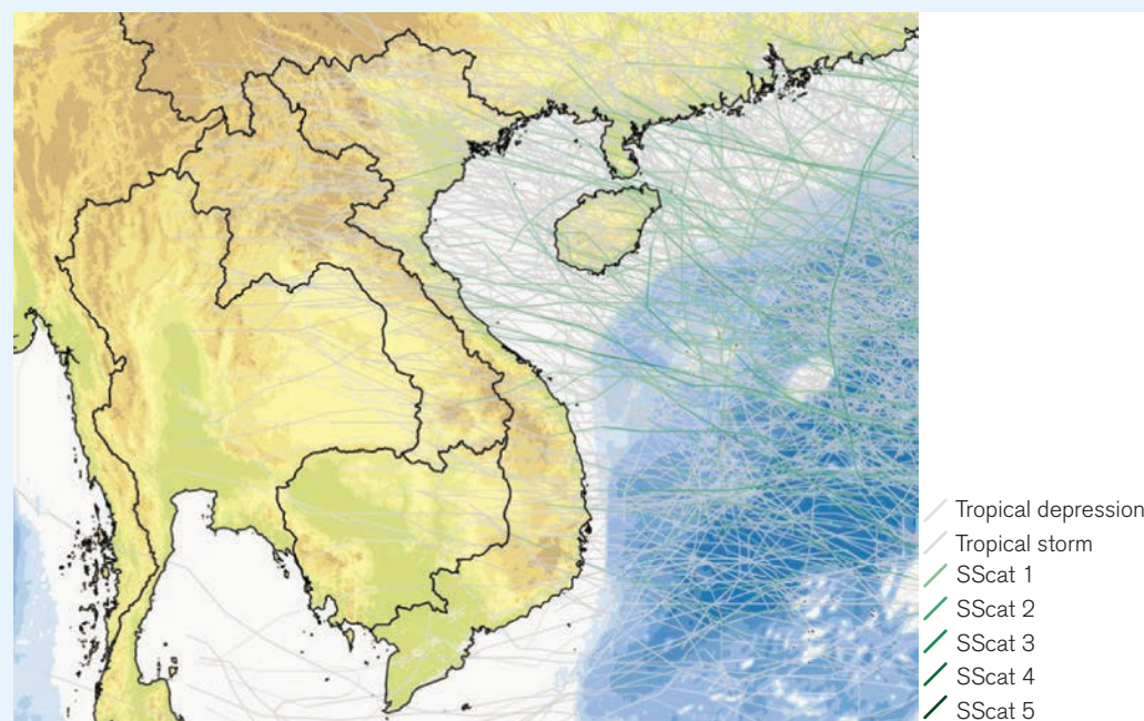
FIGURE 11. Historical cyclone tracks over Vietnam (1970–2015) 37
