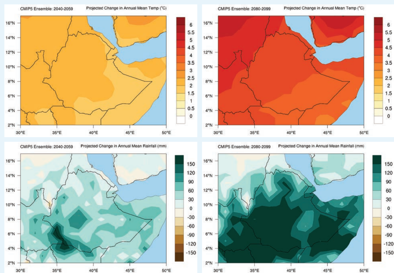
FIGURE 4. CMIP5 ensemble projected change (32 GCMs) in annual temperature (top) and precipitation (bottom) by 2040–2059 (left) and by 2080–2099 (right), relative to 1986–2005 baseline under RCP8.5 25
