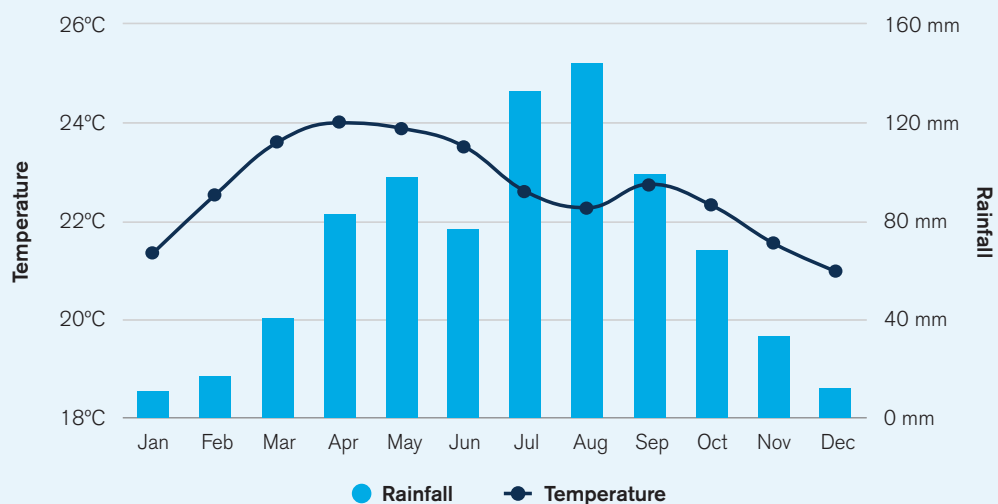
FIGURE 2. Average monthly temperature and rainfall for Ethiopia, 1901–2016 18
