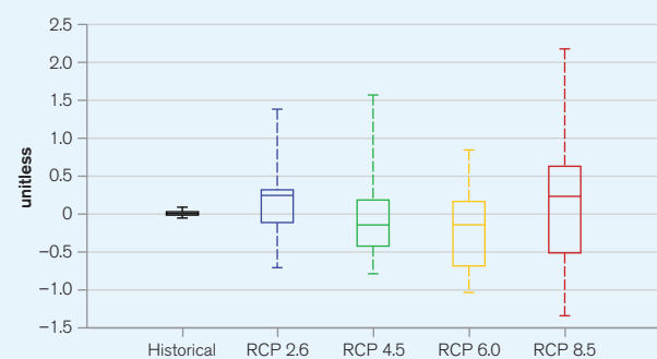
FIGURE 10. Annual SPEI Drought Index in Ethiopia for the period, 1986 to 2099 70
