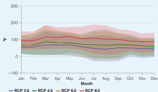
FIGURE 11. Change in Cooling Degree Days (65°F) in Ethiopia for the period 2040–2059 78
