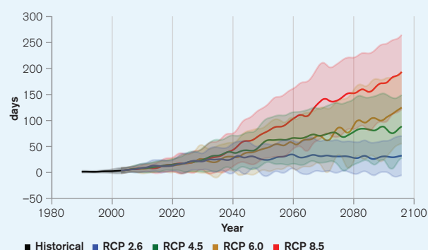
FIGURE 12. Warm Spell Duration Index in Ethiopia for the period 1986 to 2099 79
