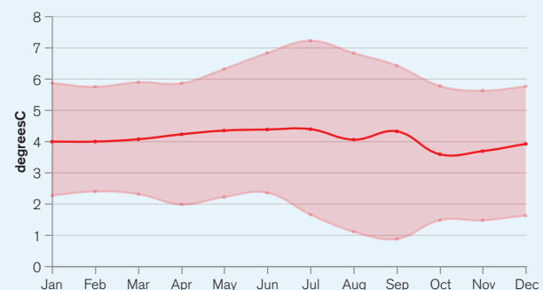
FIGURE 9. Average daily max temperature for Ethiopia 61
