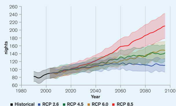
FIGURE 14. Number of Tropical Nights (Tmin >20°C) 85
