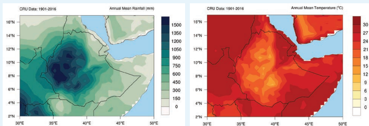
FIGURE 3. Map of average annual precipitation (left); annual temperature (right) of Ethiopia, 1901–2016 19
