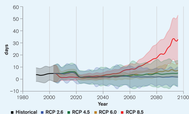
FIGURE 13. Days with a Heat Index >35°C 84
